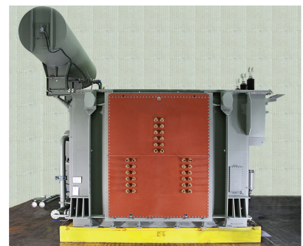
The highest rated 300 MVA EAF power transformer, built for MMK / ATAKAS in 2010
