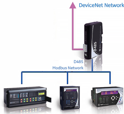
Connect multiple Modbus devices to a DeviceNet network
