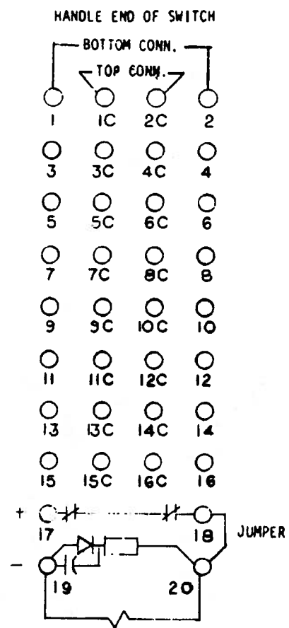
INTERNAL CONNECTIONS
