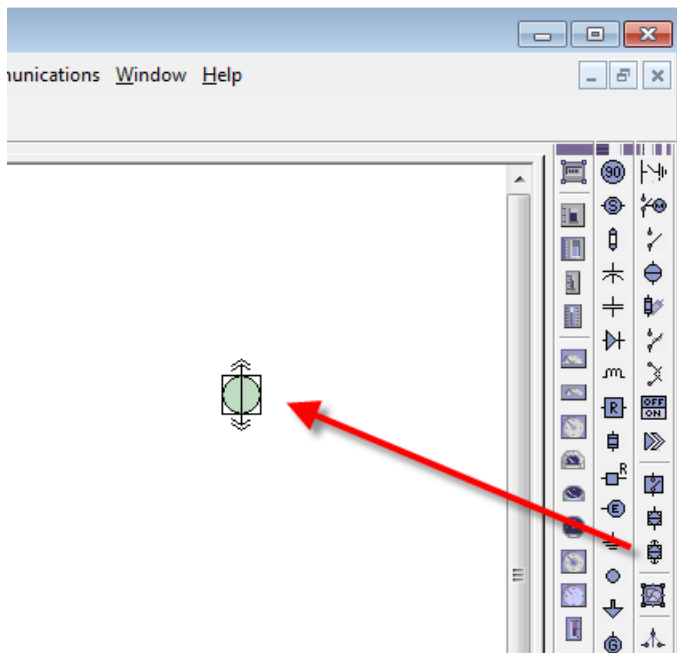
Figure 97: Add breaker
