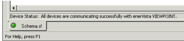
Figure 50: Schema indicator
