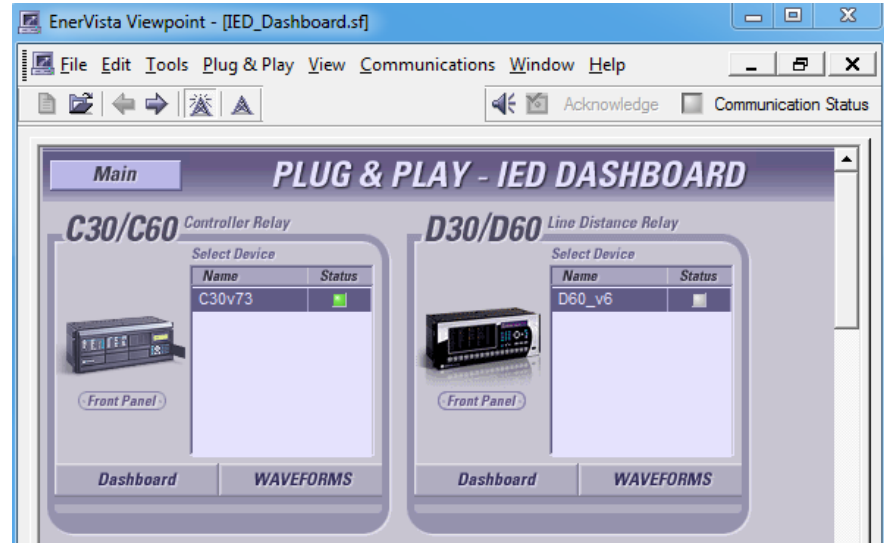
Figure 73: IED Dashboard
