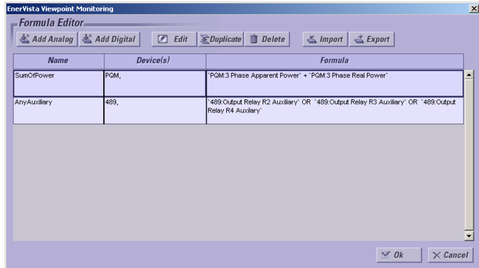
Figure 67: Formulas
