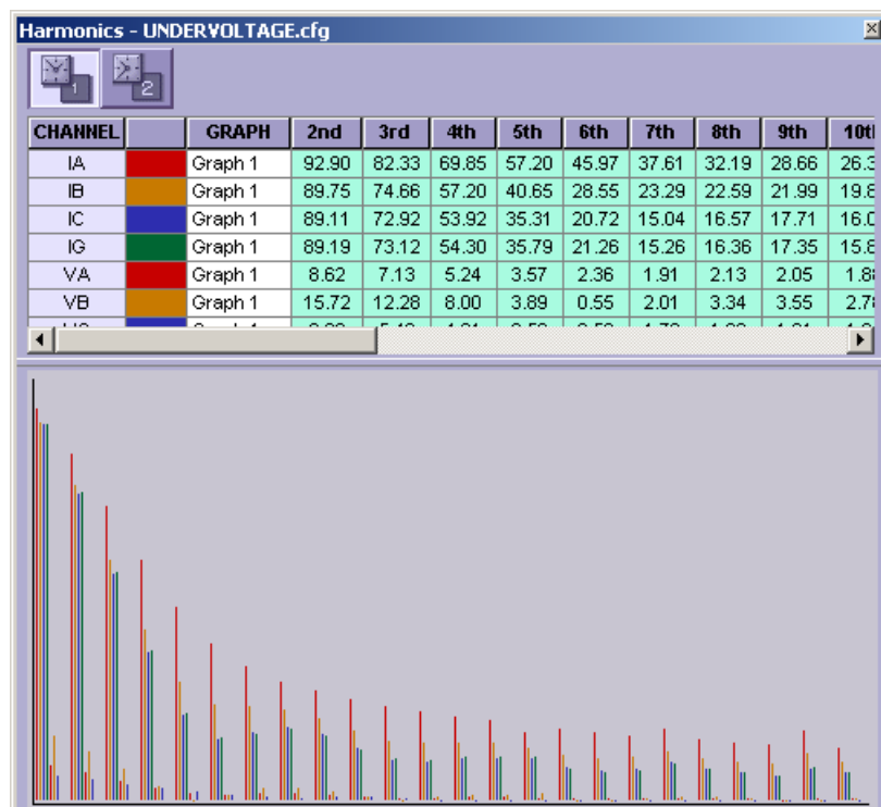
Figure 167: Harmonics window
