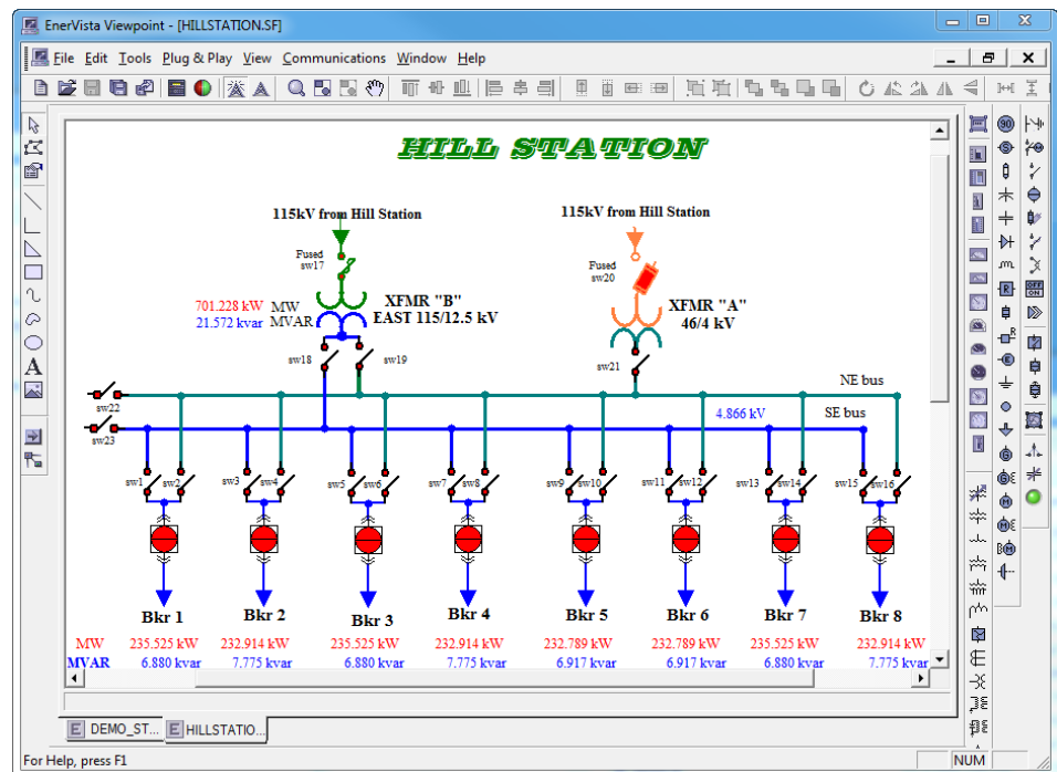
Figure 91: Example of one-line diagram
