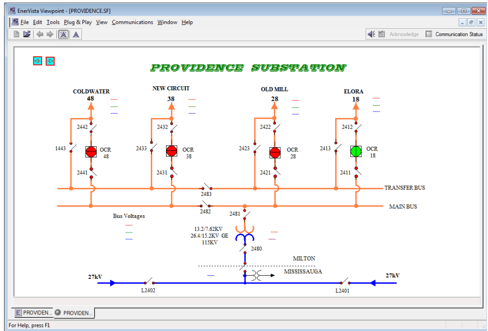
Figure 112: Example of same schema in One-Line Viewer
