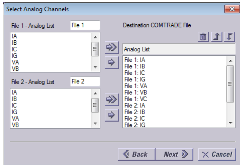
Figure 170: Analog channels
