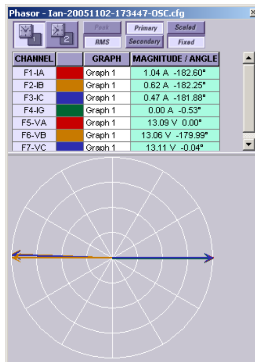
Figure 166: Phasor window
