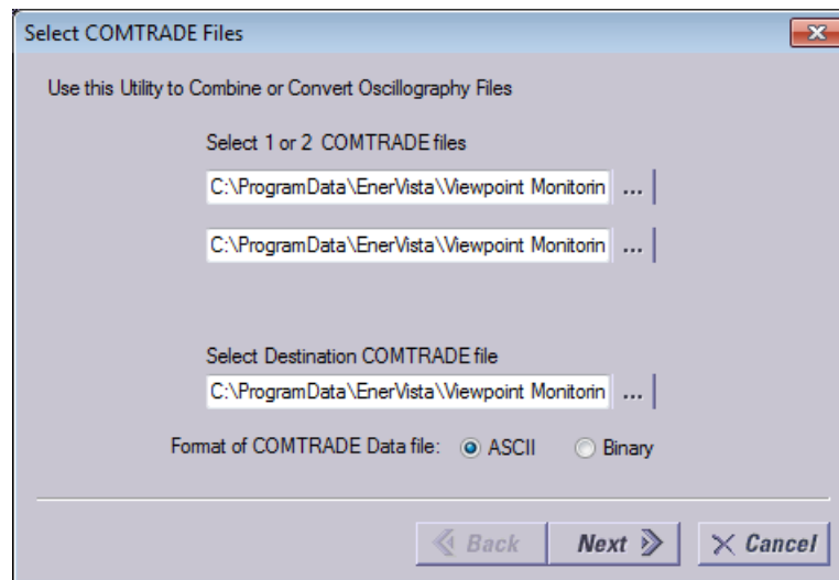
Figure 169: Merging files
