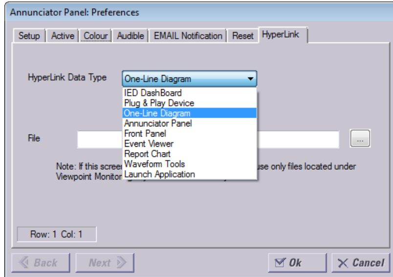
Figure 133: Hyperlink tab
