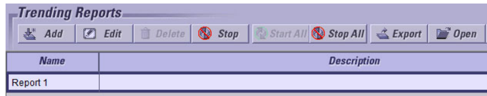
Figure 152: Export button
