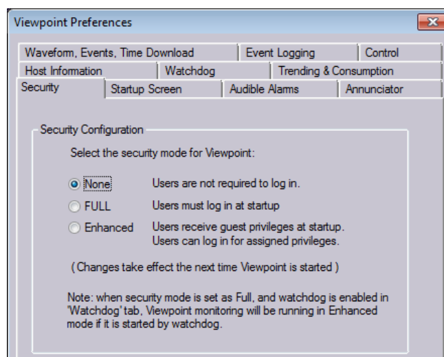
Figure 30: Security tab
