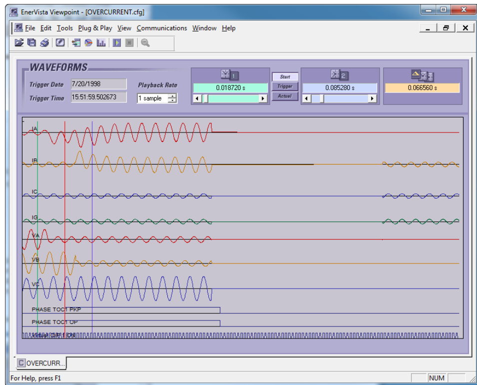
Figure 159: Demonstration file
