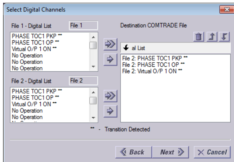
Figure 171: Digital channels
