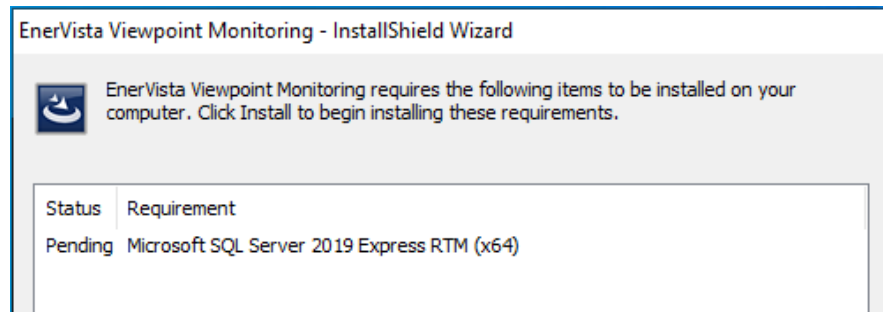
Figure 2: Installation Wizard
