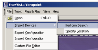
Figure 89: Importing devices
