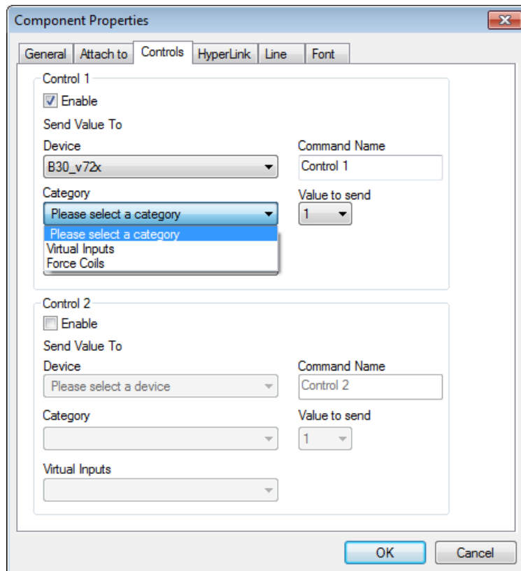
Figure 108: Controls tab
