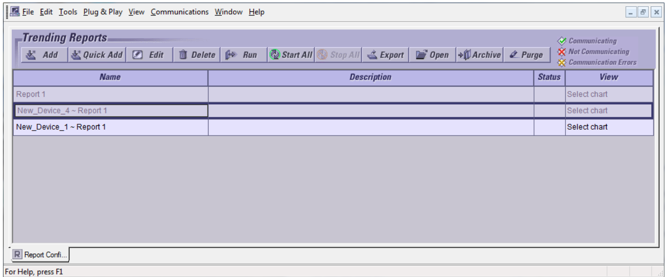
Figure 146: New report
