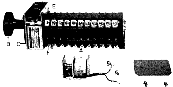
Fig. 1. Type HSA relay with cover and coil assembly removed
