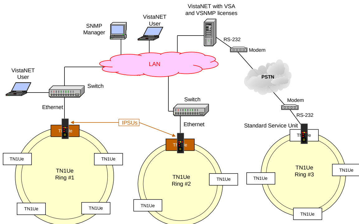
Figure 3: Control of two separate TN1Ue systems with IPSUs installed
