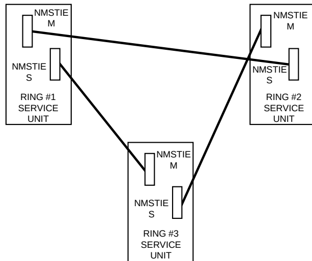
THREE-RING NMS-TIE CONNECTION
