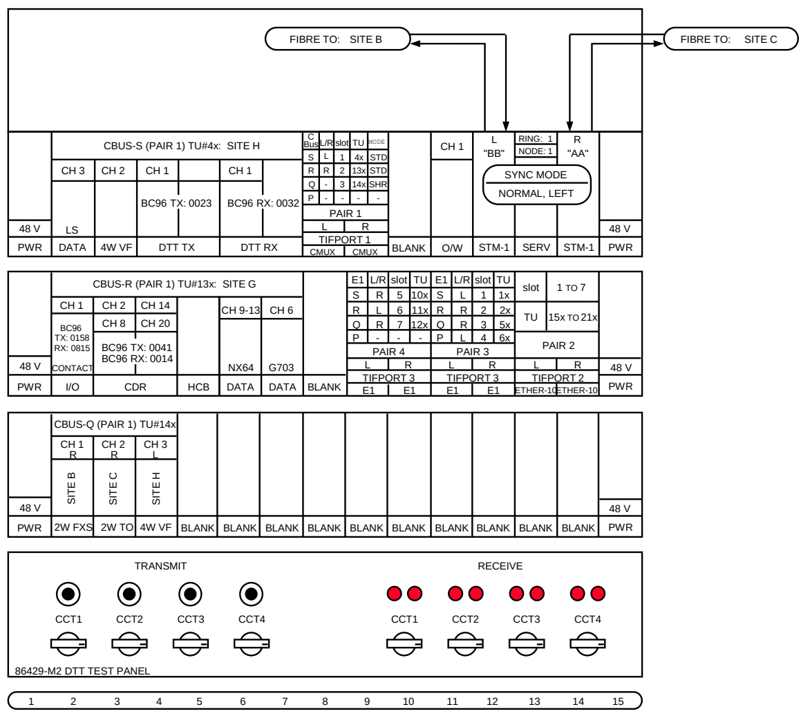
Figure 7: Typical Rack Layout for a TN1Ue SDH Node
