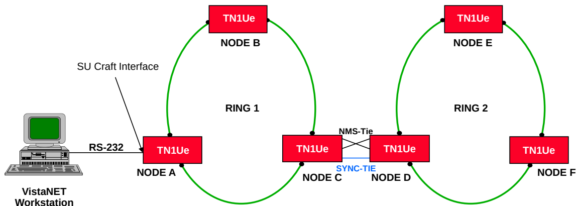
Figure 1: Visibility of two TN1Ue rings on one VistaNET workstation
