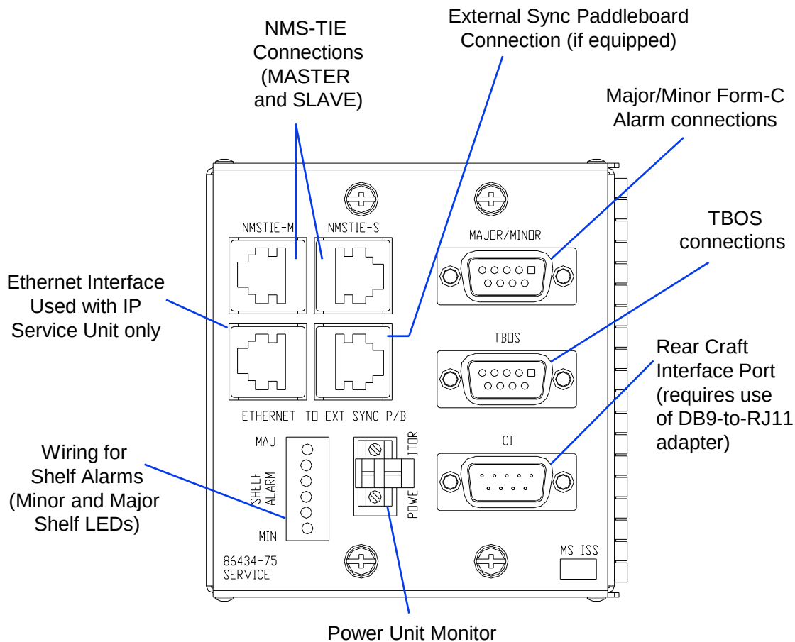
Figure 9: 86434-75 Service Unit Paddleboard Connections
