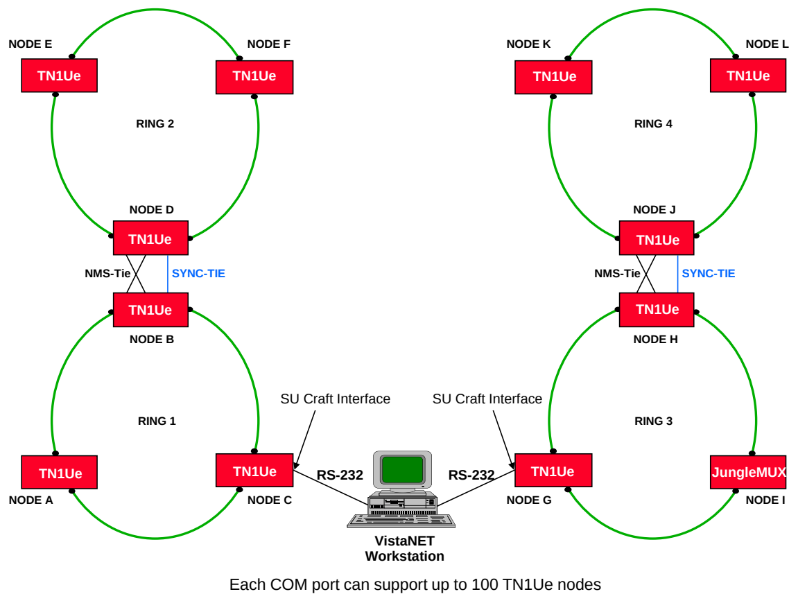
Figure 2: Visibility of two separate TN1Ue systems on one VistaNET PC
