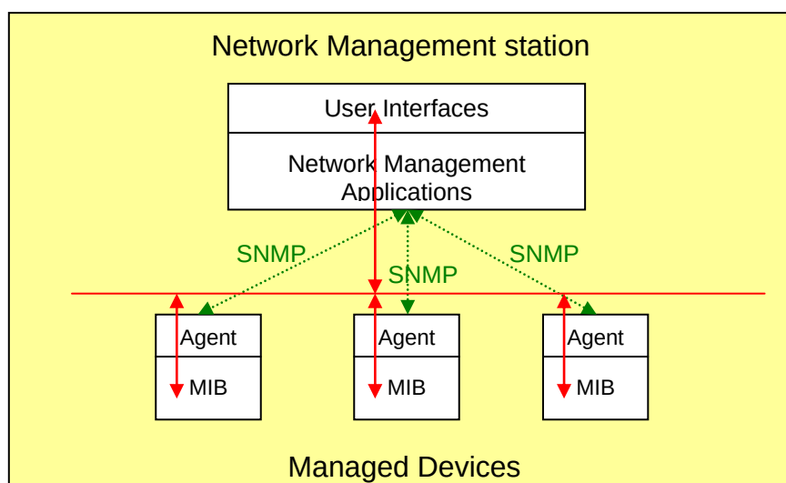
Figure 16: SNMP Model
