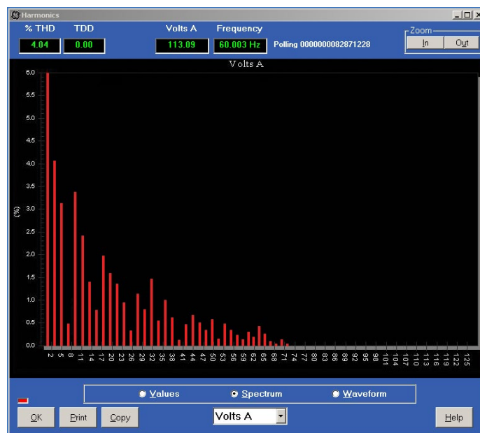
Harmonic Spectrum
