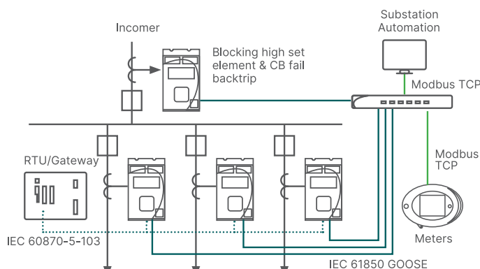
Mixed Communication Protocols: Application Example
