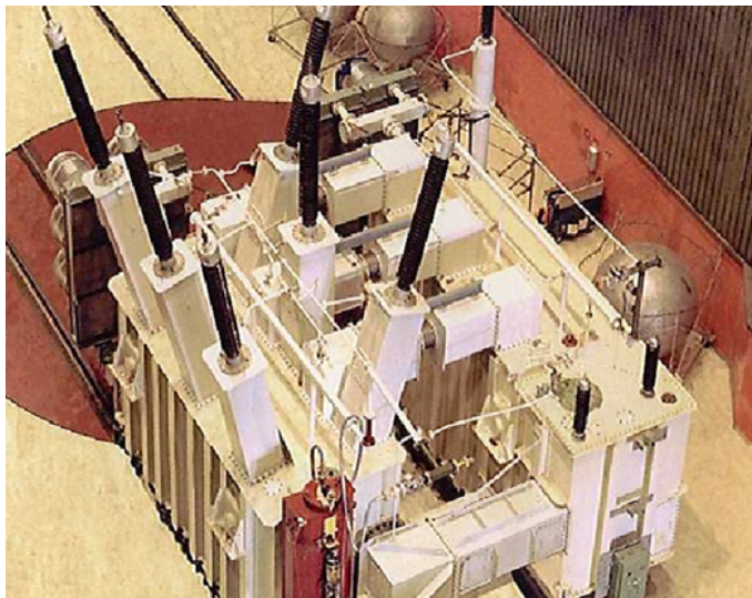
312 MVA 225 kV two-tanks, dual-core phase-shifting transformer
