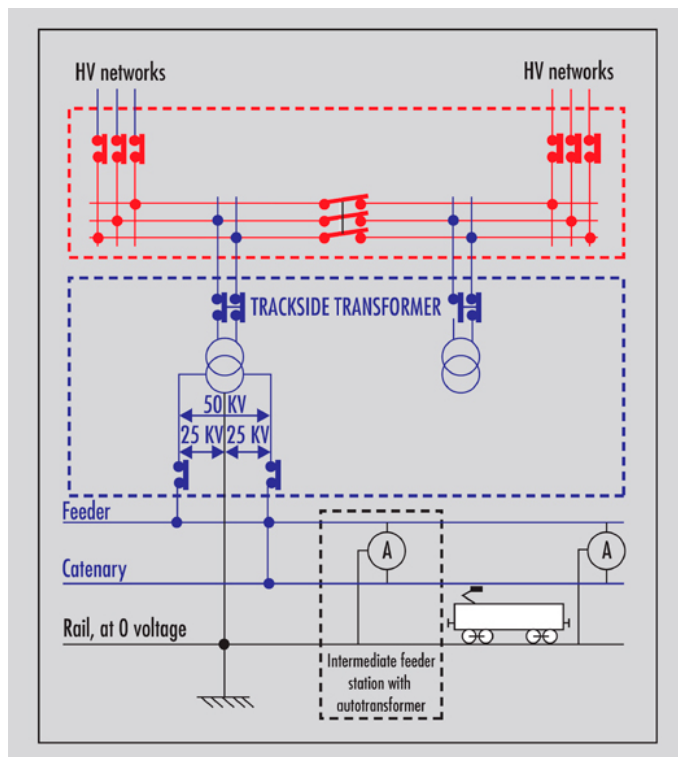
25 kV feeder system with a 220 kV / 2×25 kV trackside transformer and autotransformer for SNCF TGV lines (France)
