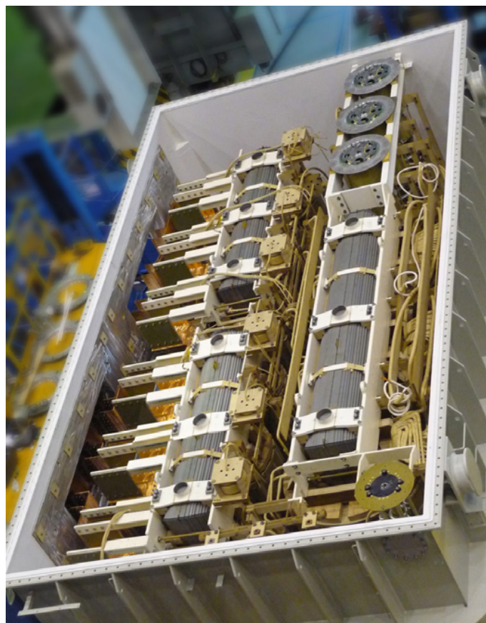
Active parts of a combined rectifier transformer to be housed in a common tank
