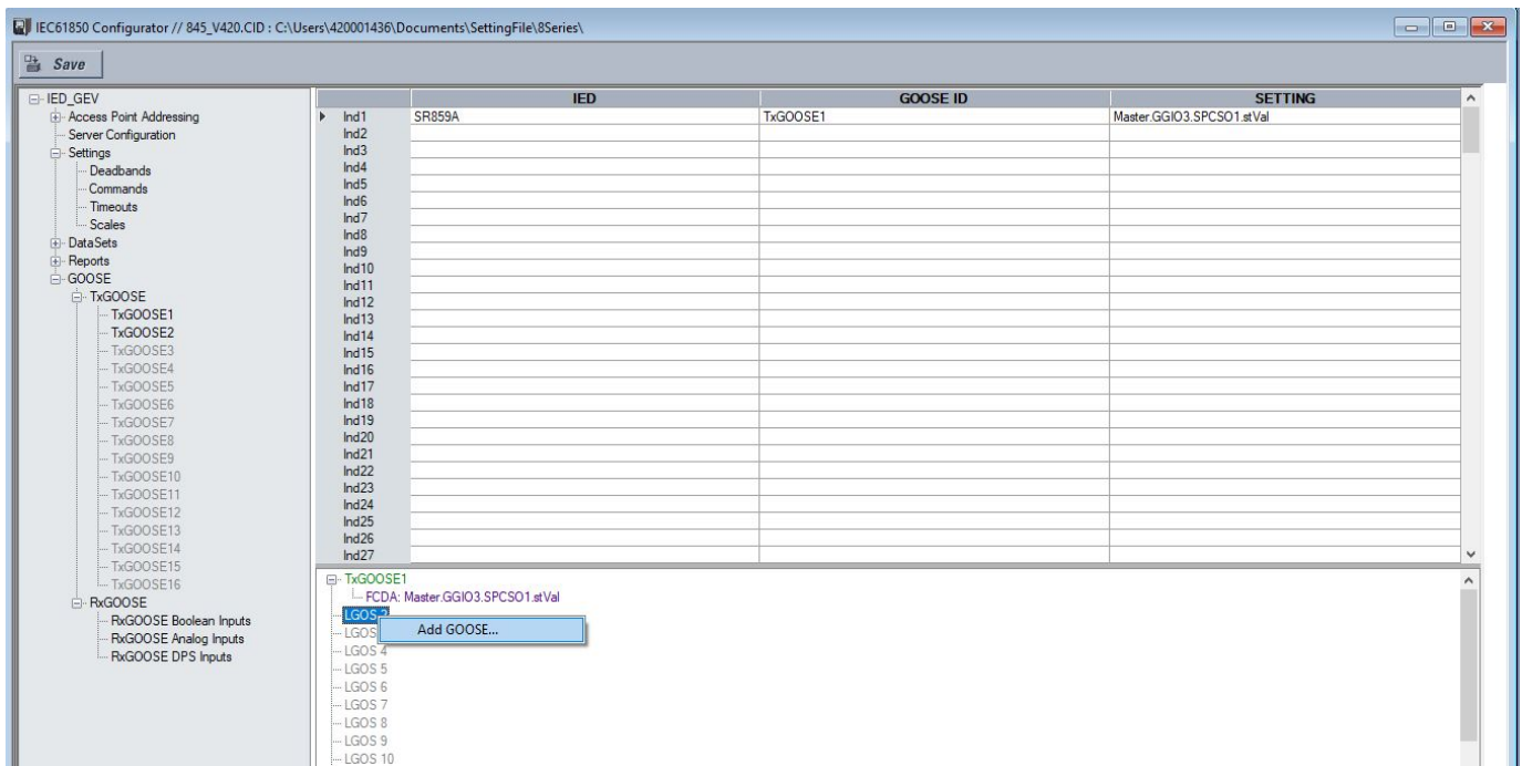
Figure 5: RxGOOSE Screen
