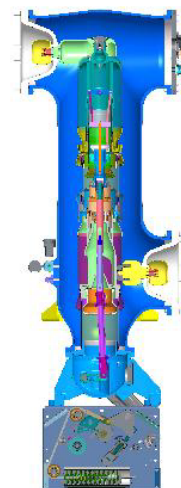
Circuit Breaker up to 420 kV 1-Pole Operated
