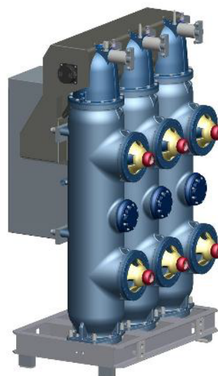
Circuit Breaker up to 145 kV 3-Pole Operated
