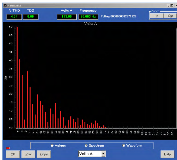
Harmonic Spectrum
