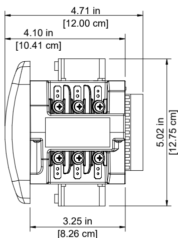
EPM 7000P Meter Side Dimensions
