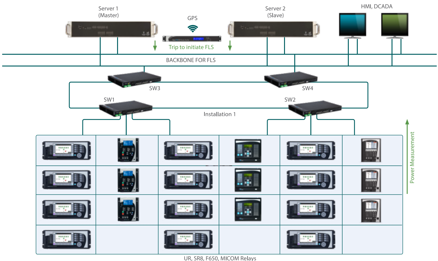
Example of Fast Load Shedding Architecture
