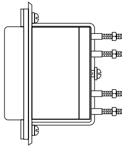
BC semi-flush mounting with cover
