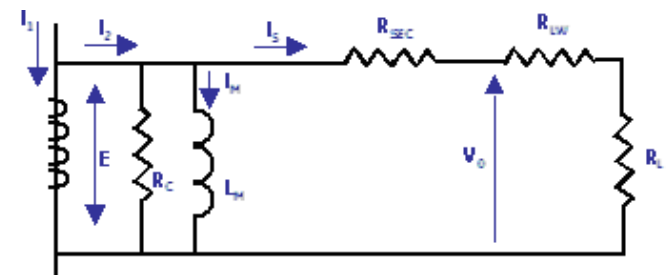
Figure 2 – Basic Magnetic Circuit
