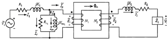
Figure 3 – Non-Ideal Magnetic Circuit
