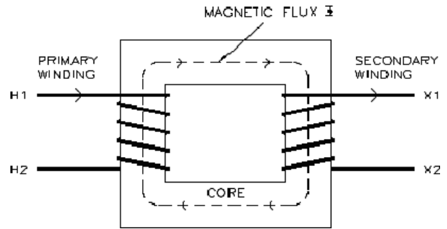
Figure 2 – Basic Magnetic Circuit
