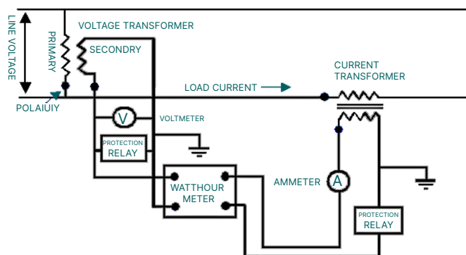
Figure 1 – Common uses of instrument transformers
