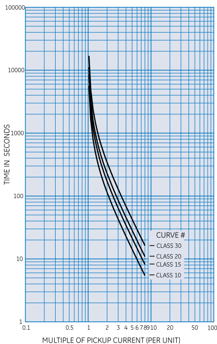
NEMA compatible time/current overload curves.
