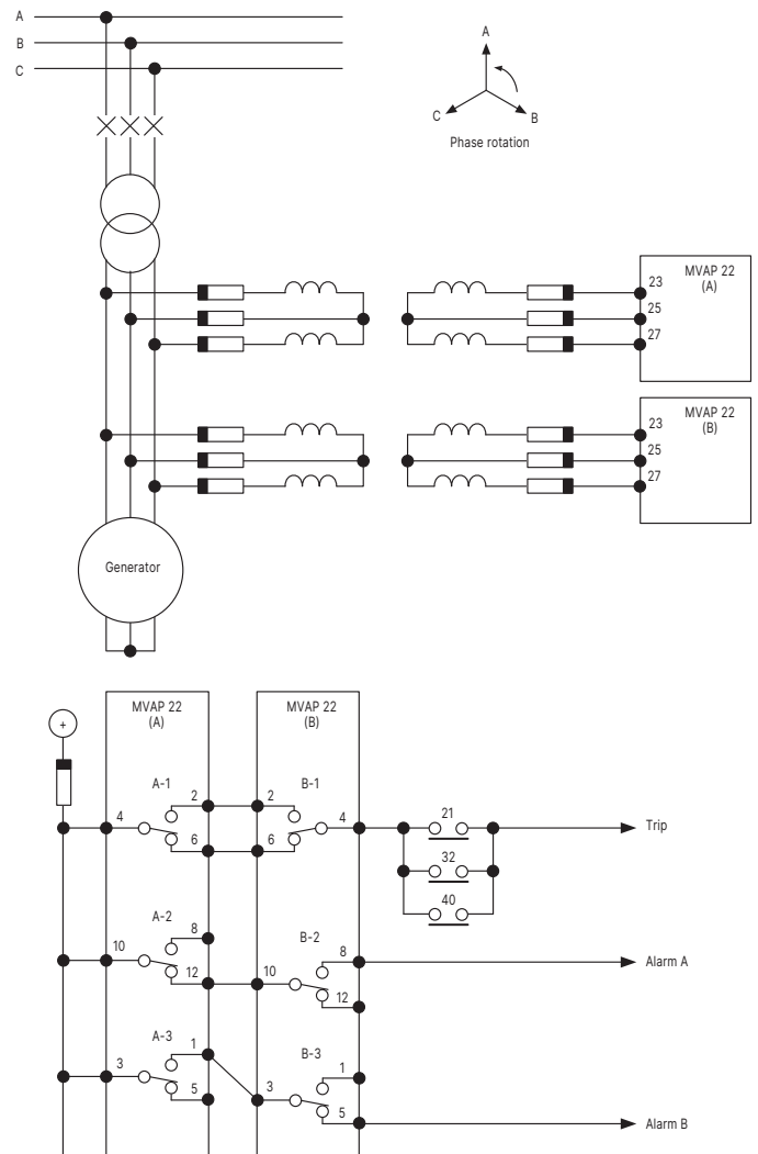
Figure 3: Application diagram: Connection of MVAP 22 relays to provide an equivalent function to a voltage balance relay on generator VTs
