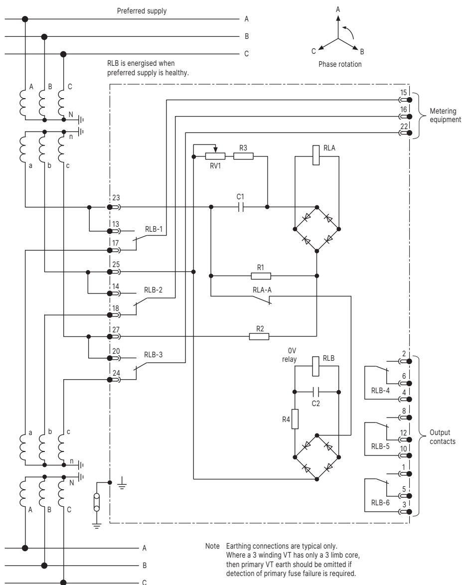
Figure 2: MVAP 22 application diagram
