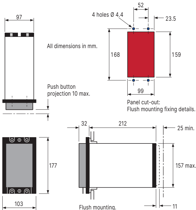
Figure 4: Case outline size 4
