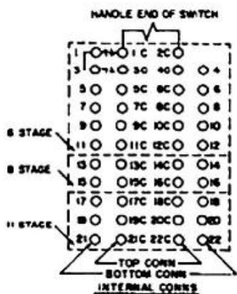
Fig. 2. HSA11 Relay Contacts
