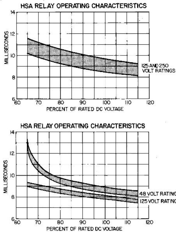
Fig. 3. Operating characteristics, 8- and 11-stage HSA relays
