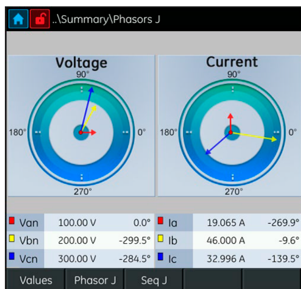
Phasor view for effective monitoring, commissioning & troubleshooting
