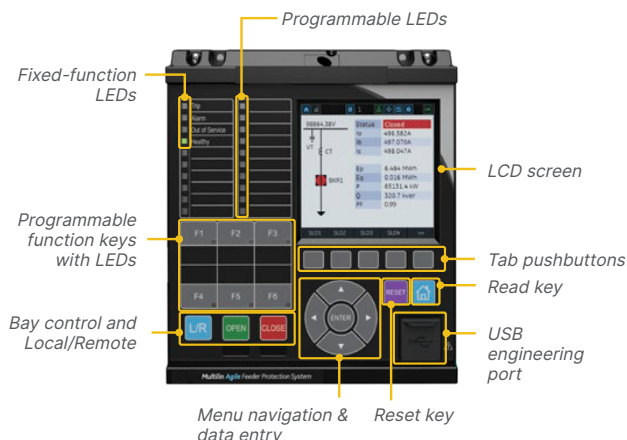
Front panel interface 30TE (6") - ANSI version
