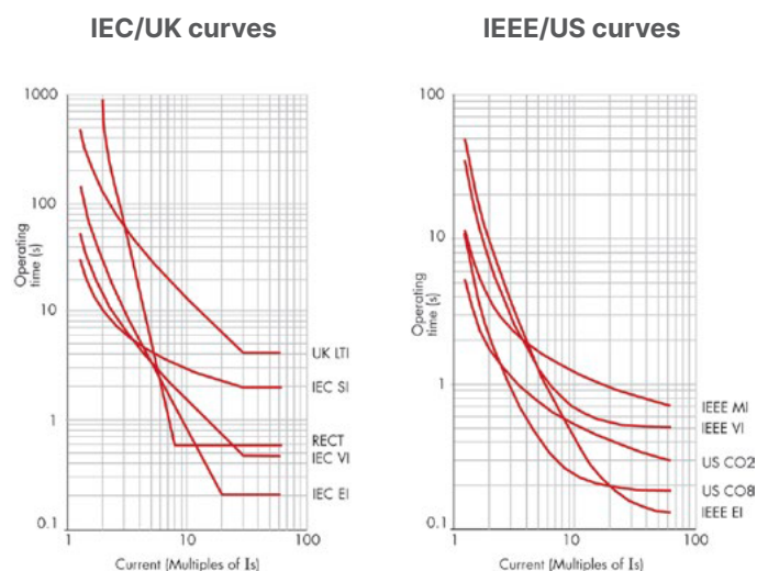
IEC and ANSI/IEEE inverse-time curve profiles
