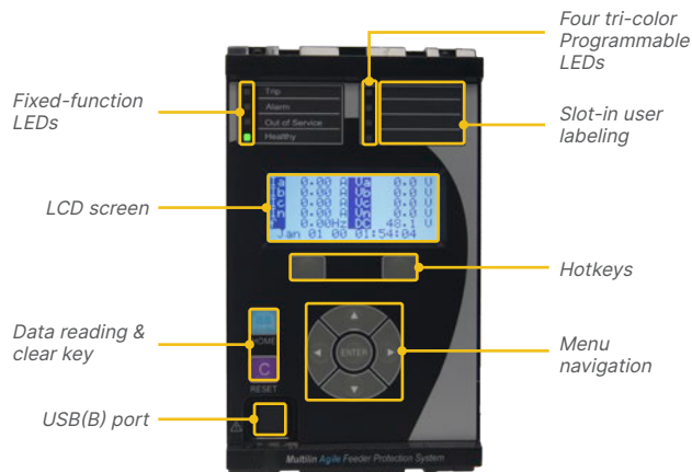
Front panel interface 20TE (4")
