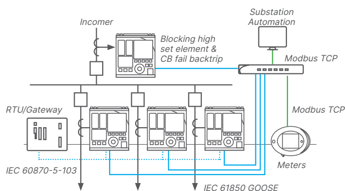
Mixed Communication Protocols: Application Example
