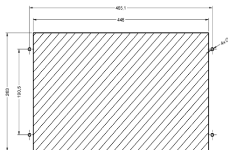
PANEL MOUNTING CUTOUT
