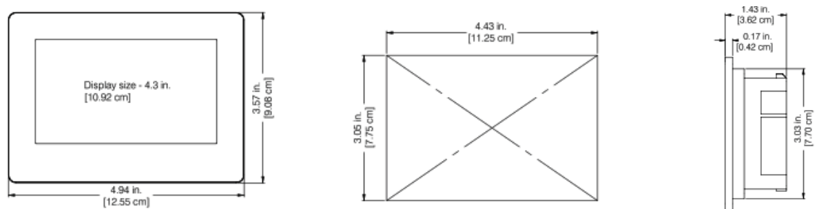
P70N Front Dimensions
