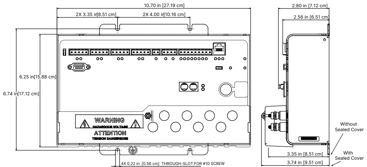
EPM 9700 Front Dimensions
