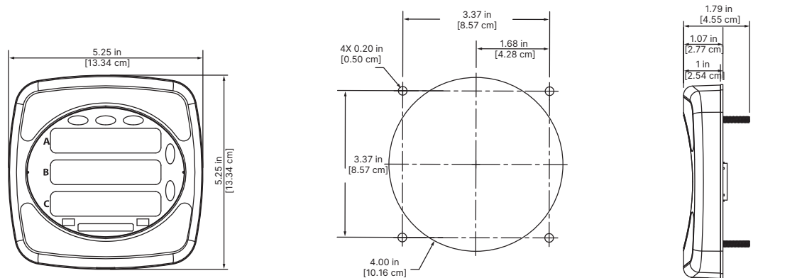
P40NPLUS Front Dimensions
