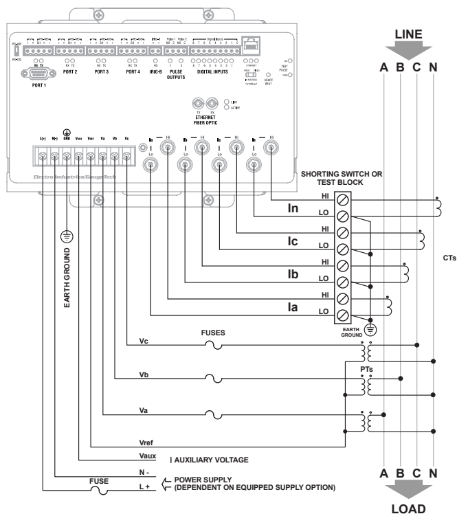
4-Wire Wye, 3-Element Direct Voltage with 4 CTs
