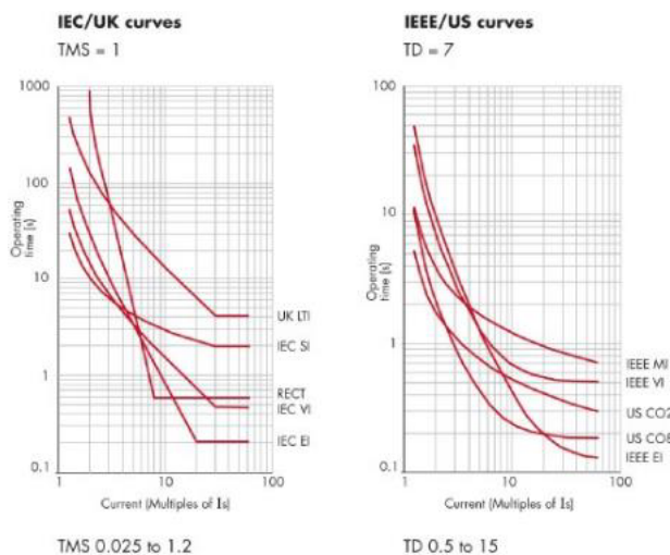
IEC and ANSI/IEEE inverse-time curve profiles
