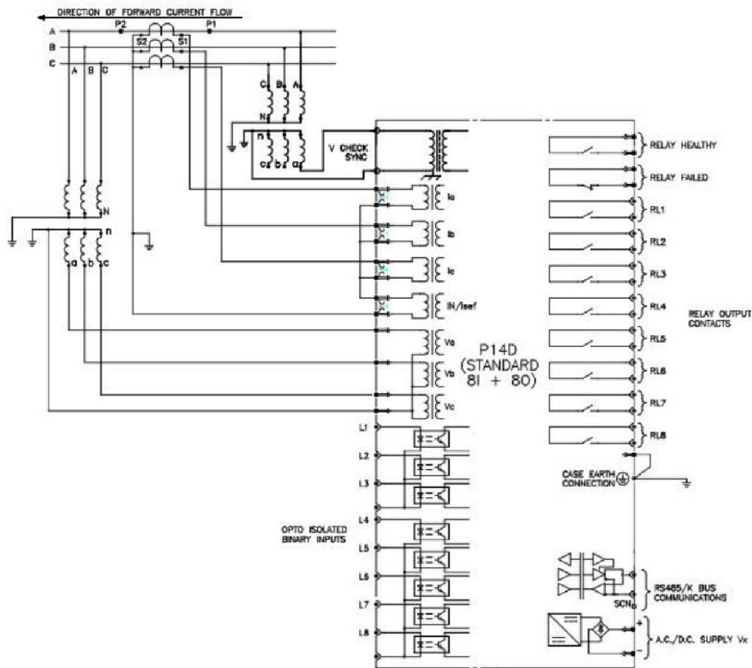
P40 Agile standard hardware (P14D)
