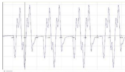
Typical current waveform trace recorded for a downed conductor
