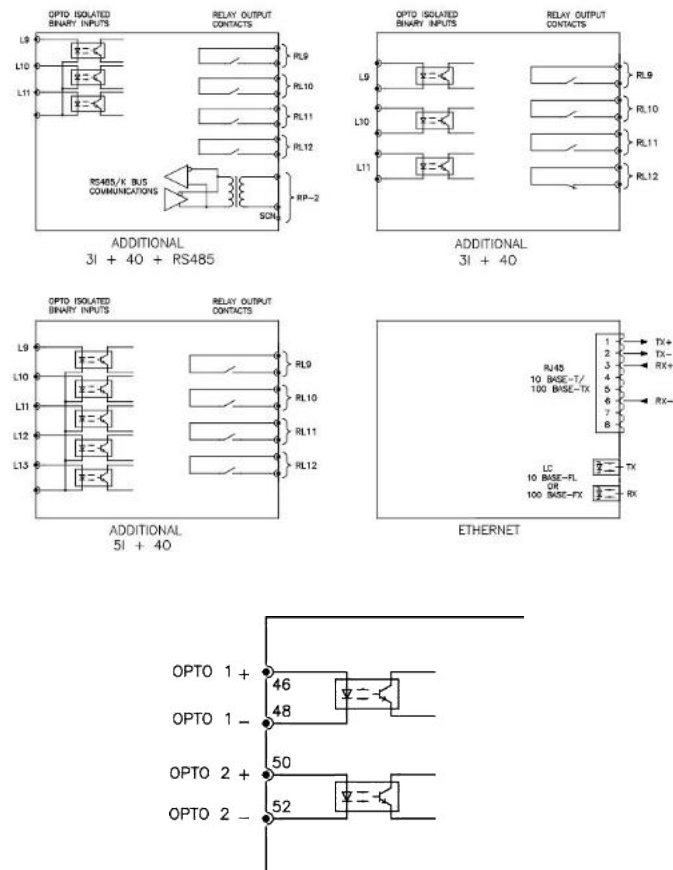
Example hardware options available in case size 30TE
