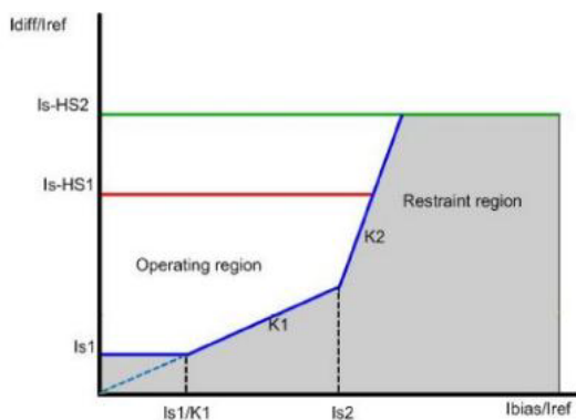
Figure 1: Biased differential protection characteristics
