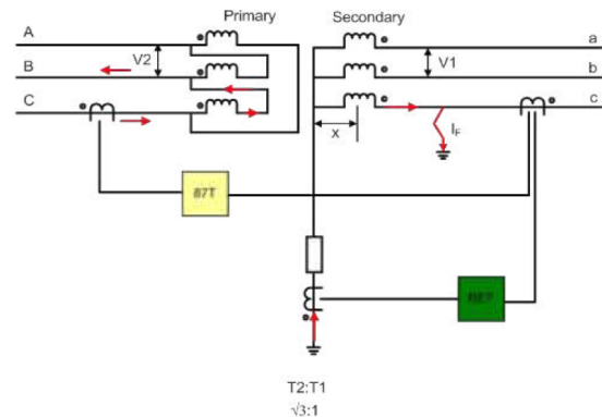
Figure 2: Restricted Earth Fault application
