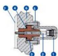
Fig. 22: Power Factor Tap (25 to 69 kV)
