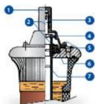
Fig. 24: Bushings' head 25 to 161 kV
