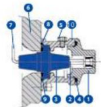
Fig. 23: Voltage Tap (115 to 765 kV)
