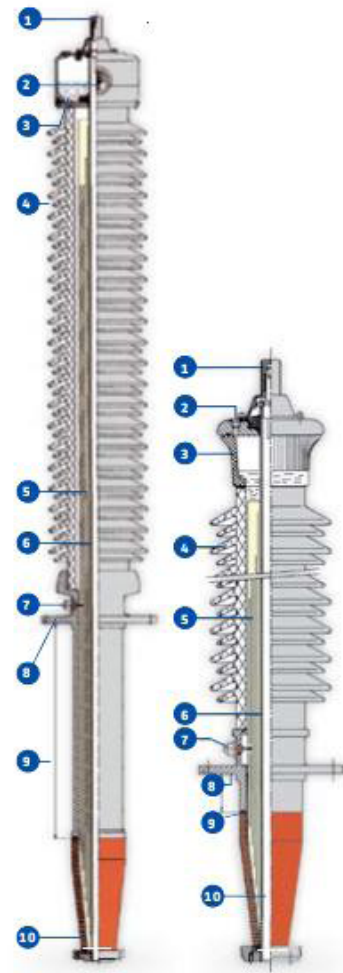
Fig.1: Bushings at 245 kV to 1050 kV
