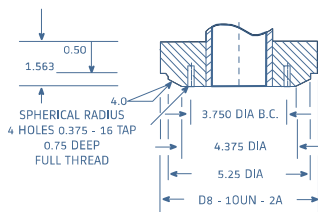
Fig. 19: Bottom terminal type 3
