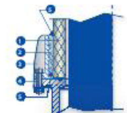
Fig. 11: Cemented Porcelain
