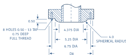
Fig. 20: Bottom terminal type 4
