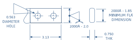
Fig. 17: Bottom terminal type 1
