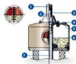
Fig. 25: Bushings' head 230 to 765 kV
