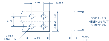
Fig. 18: Bottom terminal type 2
