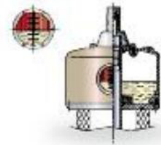
Fig. 8: Head of bushings 230 to 765 kV
