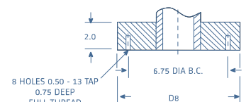
Fig. 21: Bottom terminal type 5
