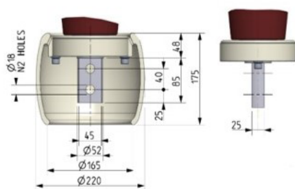
Fix - conductor n2 holes 123 - 245 kV
