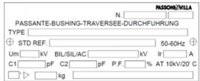
Fig. 2: Nameplate
