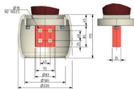
Fix - conductor n4 holes 123 - 245 kV
