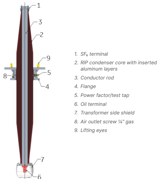
Fig. 1: POBR, typical cross section
