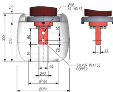
Fix - conductor n2 holes 420 kV
