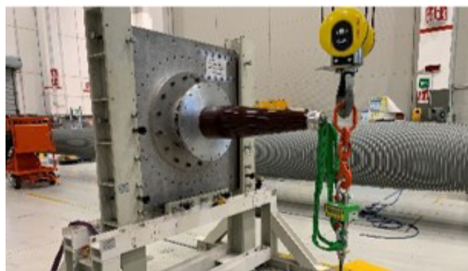
Fig. 7: Cantilever Test
