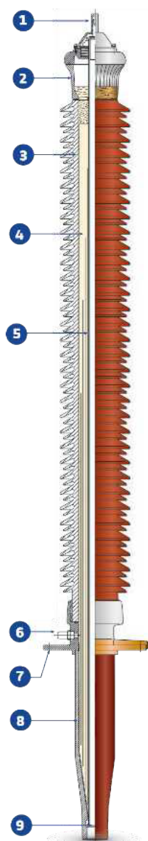
Fig. 1: Bushings 52 to 170 kV Heavy Cantilever load
