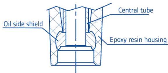
Fig. 4: Oil side shield embedded in the epoxy resin housing
