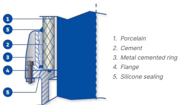
Fig. 5: Cemented porcelain
