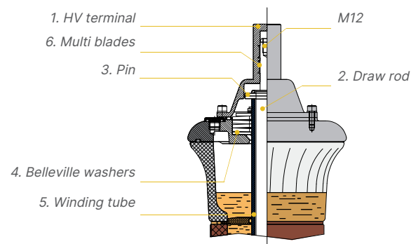
Fig. 8: 52-170 kV bushing head: draw rod connection
