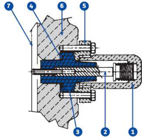
Fig. 3: Power Factor Tap
