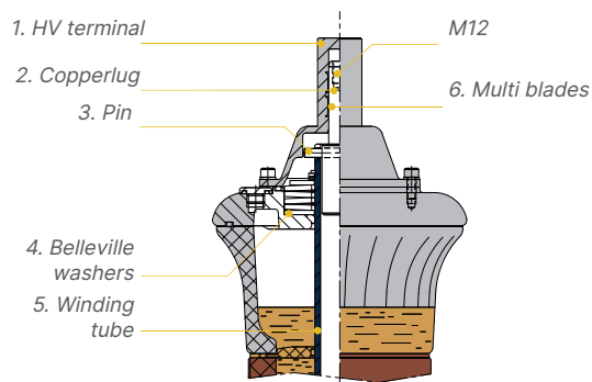
Fig. 7: 52-170 kV bushing head: draw lead connection
