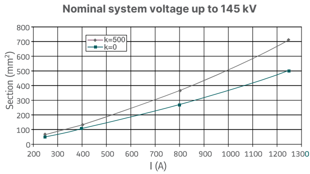
Fig. 9: Draw lead conductor sections
