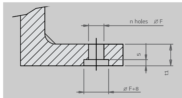
Fig. 13: Flange fixing holes
