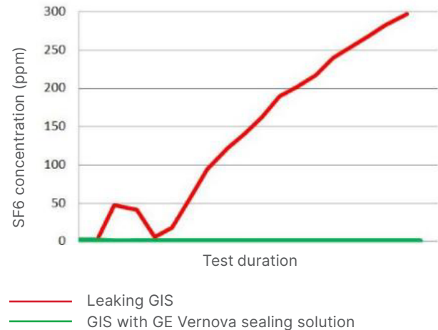
Figure 2 - Tightness test at customer site
