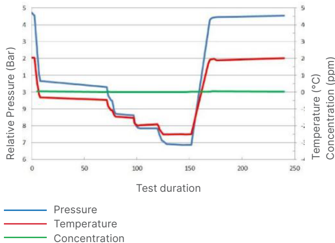
Figure 1 - Thermal cycling test in lab
