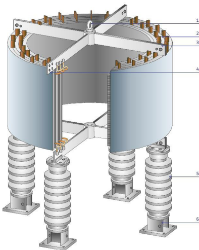
Air Core Reactor Construction
