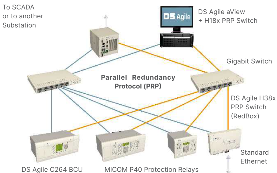
IEC 62439-3-4 PRP dual star, Ethernet-based architecture
