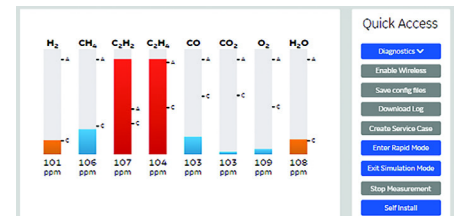
DGA 900 gas levels displayed on the local LCD screen
