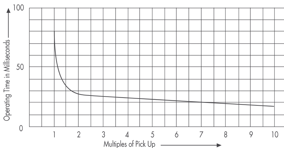
Figure 5: Time/current characteristic
