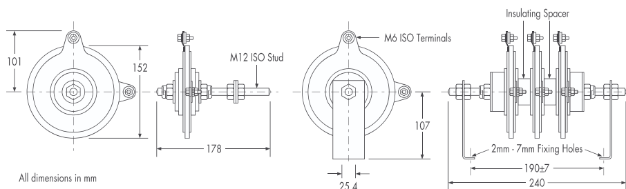
Figure 4: Outlines of external Metrosil units
