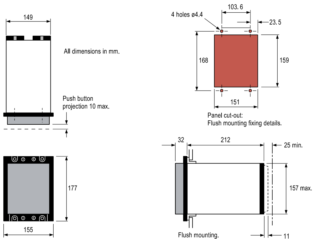
Figure 7: Case outline 30TE (size 6)
