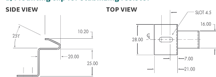
b) Stabilizing resistor
