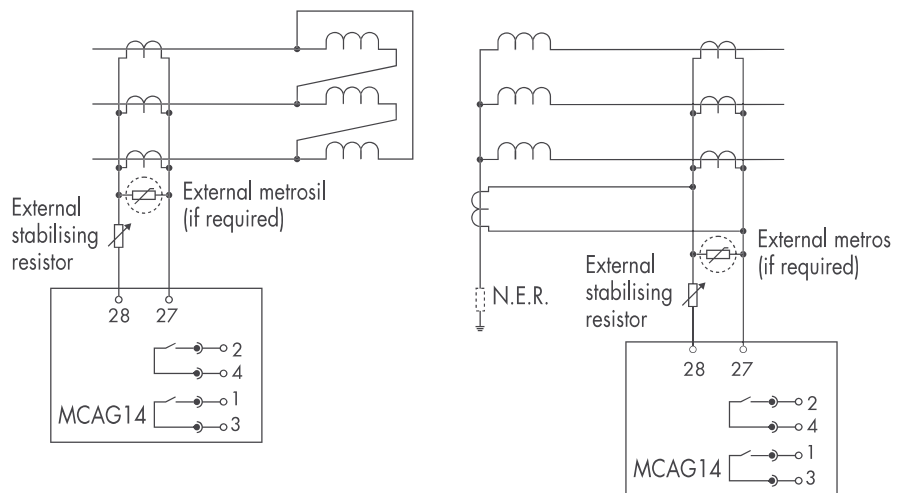
Figure 2: Type MCAG14 relays applied to restricted earth fault protection of power transformer
