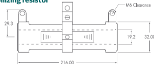
Figure 3: External stabilizing resistor assembly
