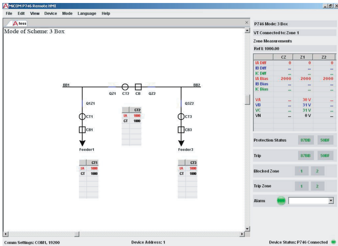
Remote HMI
