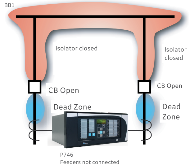
Dead zone protection
