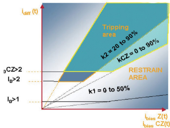
Bias differential characteristics
