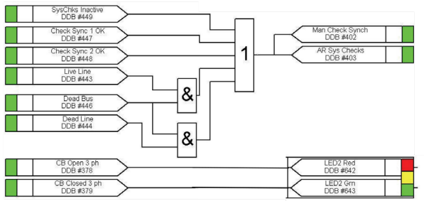
Programmable scheme logic editor (MiCOM S1 Agile)
