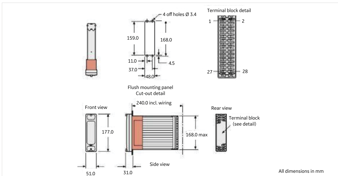
Figure 6 Mounting Details
