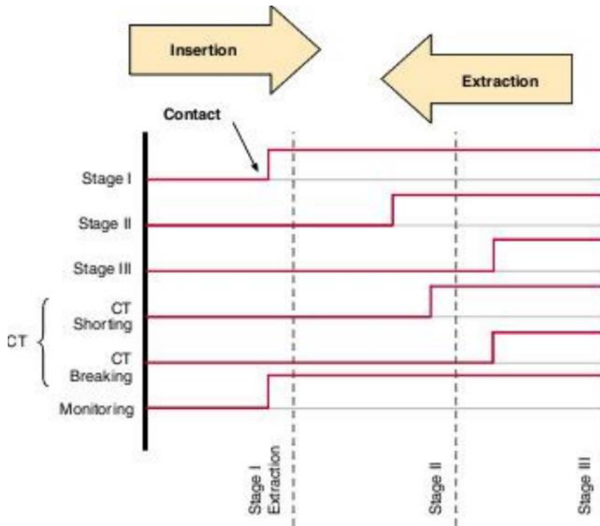
Figure 1 Sequence diagram during insertion and extraction of P992
