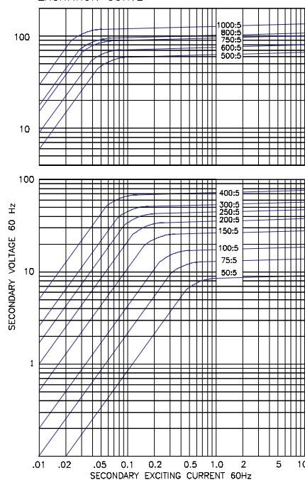
EXCITATION CURVE
