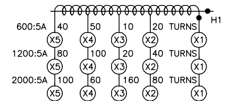
CONNECTION DIAGRAM
