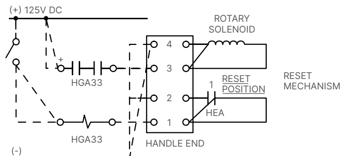
Figure 6. Typical HEA63B contact arrangement
