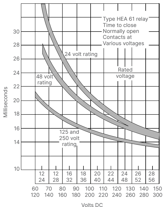
Figure 3. Typical time-voltage characteristics of Type HEA61 relay
