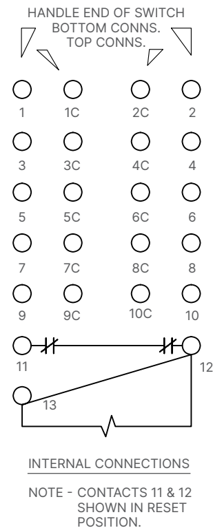
Figure 2. Typical HEA61B relay contact arrangement
