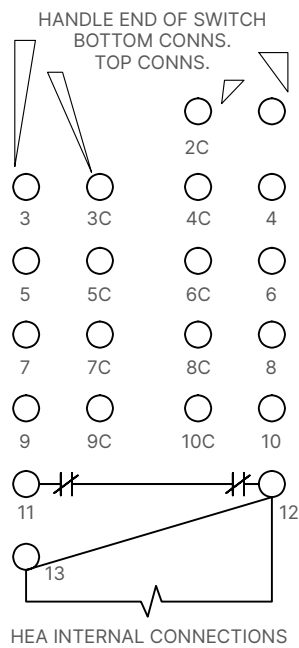
Figure 5. Typical schematic of HEA63 relay
