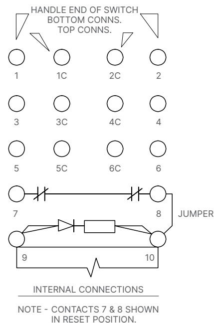
Figure 4. Typical HEA62A relay contact arrangement
