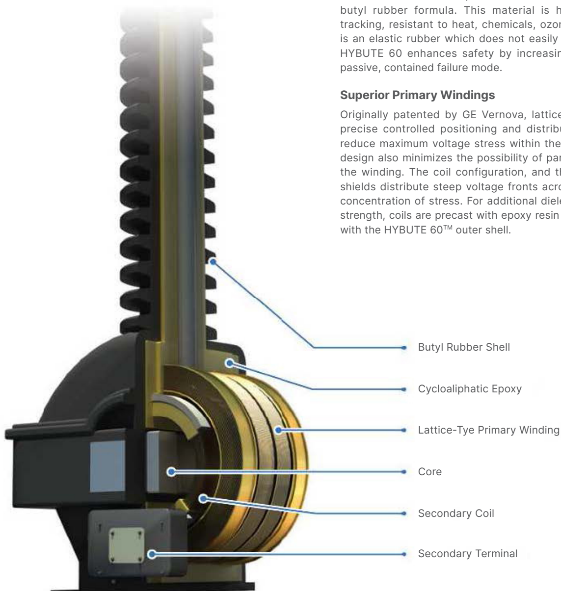
Cross-Section view of a Station-Class SUPERBUTE Vo/toge Transformer
