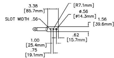
Primary Terminal
