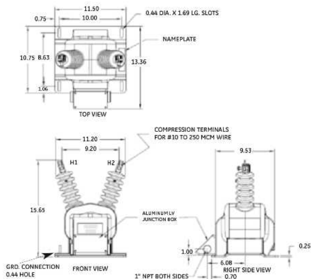
Type JVW-110C Double Bushing
