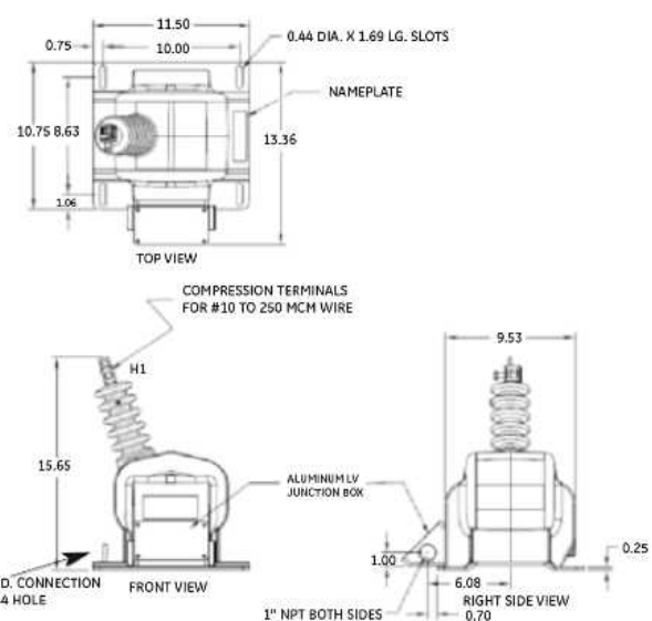
Type JVW-110C Single Bushing
