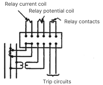
Fig. 19: Test-block connection for one current and one potential coil with connection for trip circuit
