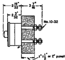
Fig. 5: 4- or 6- Pole Surface Mounted on 1 to 2 in. Panels
