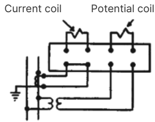
Fig. 16: Test-block connection for one current and one potential coil
