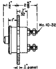
Fig. 6: Semi-flush Mounted on 1/8 in. Panel
