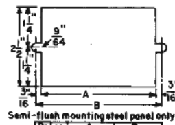
Fig. 9: Semi-flush Mounting Steel Panel only.
