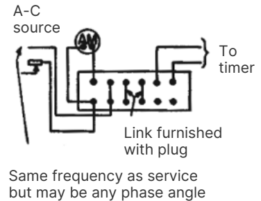
Fig. 22: Plug connection for Fig. 19 for testing relay with same or separate source
