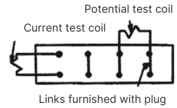
Fig. 17: Plug connection for Fig. 16 for testing one current and one potential coil in circuit
