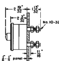
Fig. 8: 4- and 6- Pole Studs
