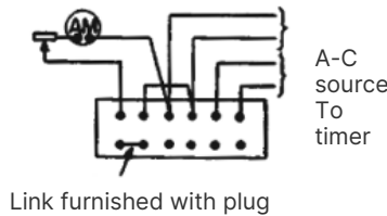
Fig. 21: Plug connection for Fig. 19 for separate test of relay with separate source
