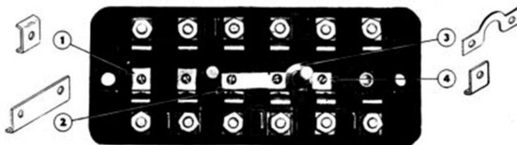
Fig. 9 shows a composite assembly of a 6-pole PK-2 test block with auxiliary contacts and jumpers, as follows:
