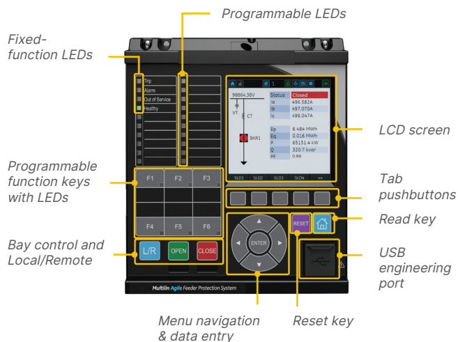
Front panel interface 30TE (6'') - ANSI version
