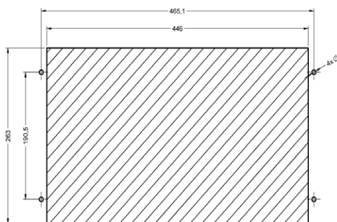
Panel Mounting Cutout
