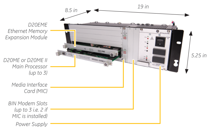
Figure 3: D20 Chassis, multiple-slots, VME type
