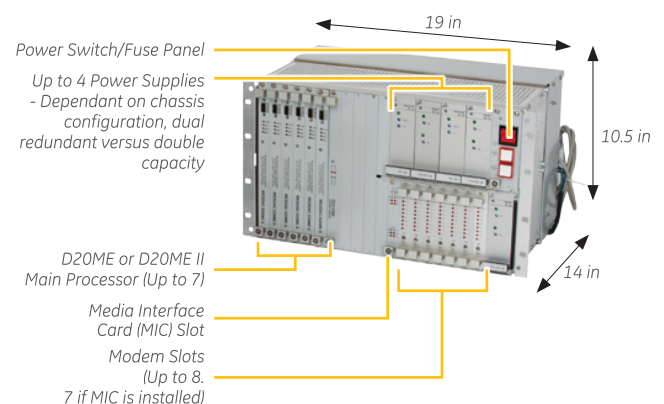
Figure 4: D200 Chassis, multiple-slots, VME-type
