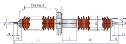
Fig. 4: Through wall bushing for normal cantilever load
