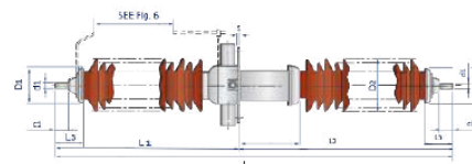
Fig. 5: Through wall bushing for heavy cantilever load
