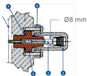
Fig. 2: Power factor tap
