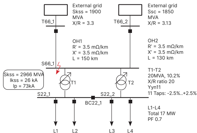
Figure 2: Simplified representation of a power network.
