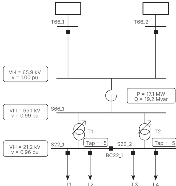
Figure 5: Voltage drop after the addition of the series reactor.
