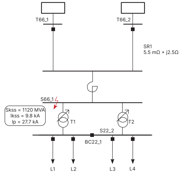
Figure 3: Simplified representation of a power network with a series reactor added.
