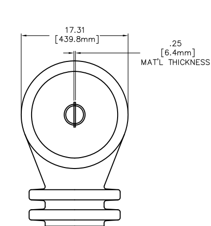
PAD CONFIGURATION FOR 800:5-1200:5 1 PAD EACH SIDE
