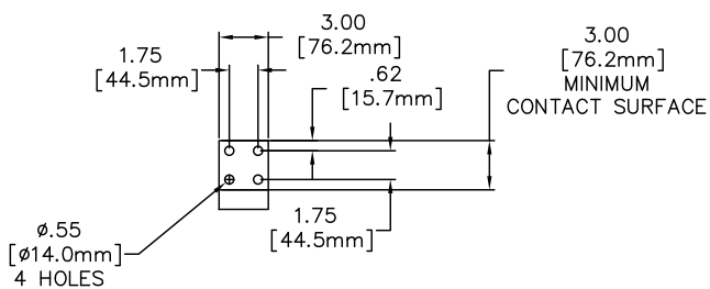
Primary - 1 PAD, up to 600A
