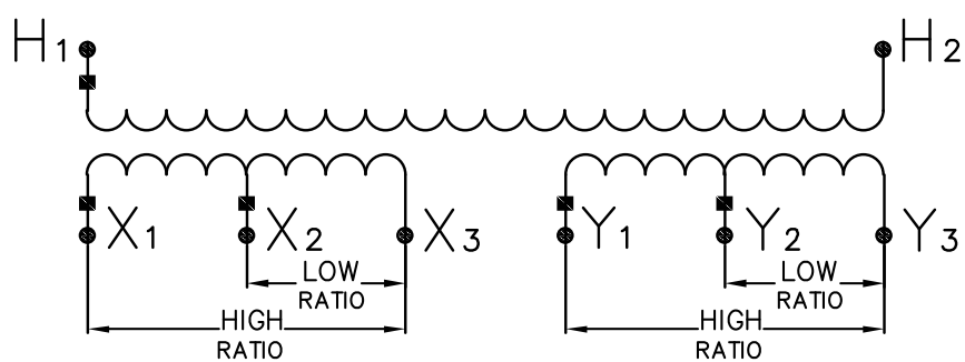
Dual-tapped secondary (Six secondary terminals)
