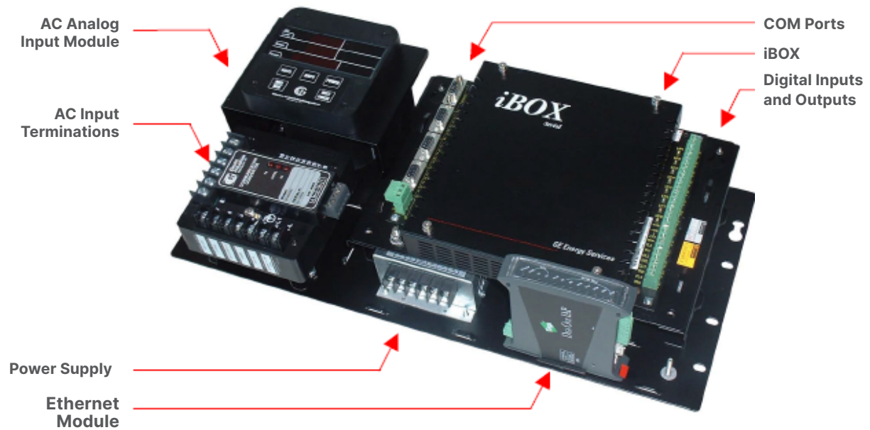
Figure 4 iBOX AC Kit
