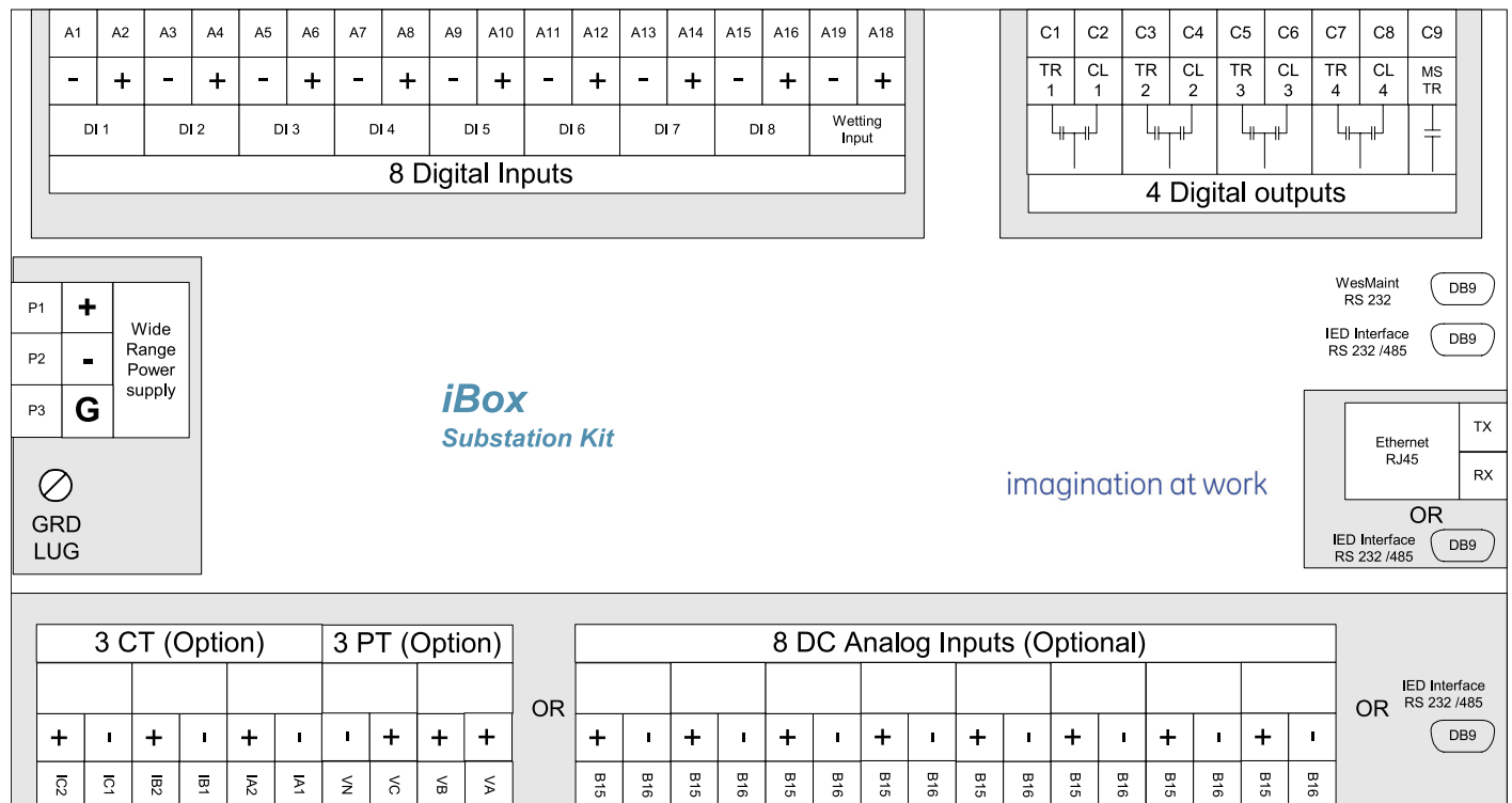
Figure 1 iBOX Kit I/O Options
