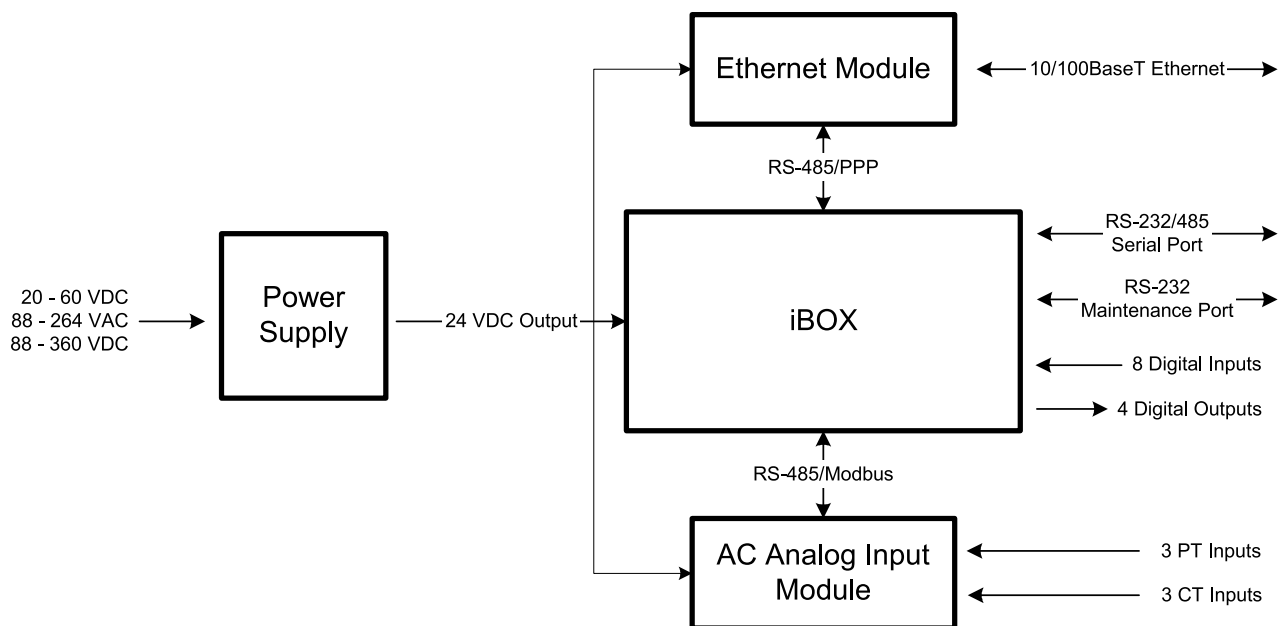
Figure 5 Fully equipped iBox AC Kit Block Diagram
