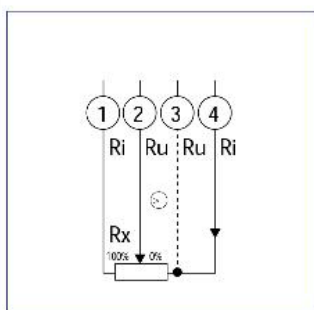
Tap Position Indicator
