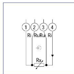
Resistance, Temperature (RTD) - 4-wire
