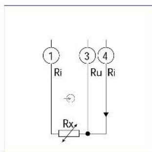
Resistance, Temperature (RTD) - 3-wire
