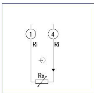
Resistance, Temperature (RTD) - 2-wire
