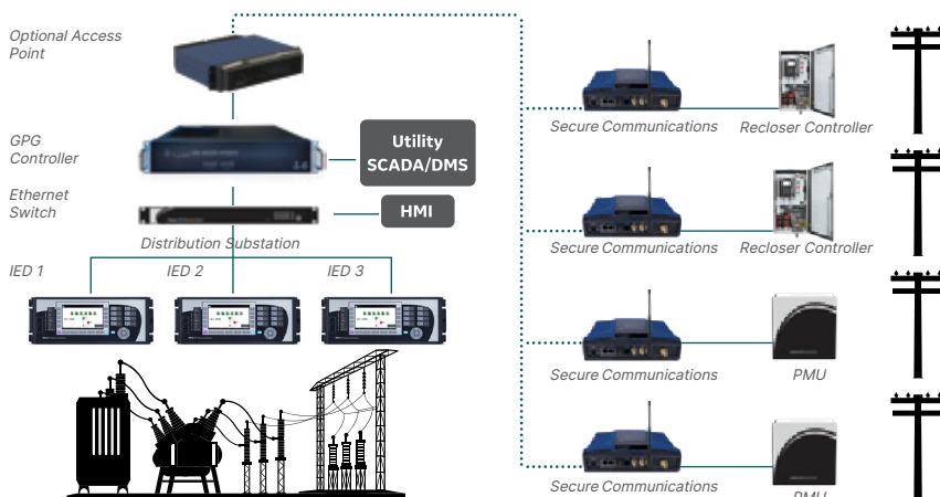
GridNode HFSP architecture
