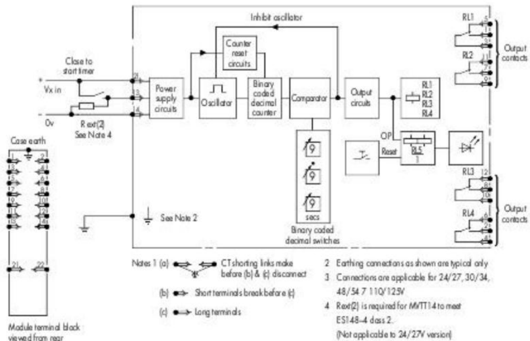
Figure 2 Application diagram: digital time delay relay type MVTT 14 (dc version)
