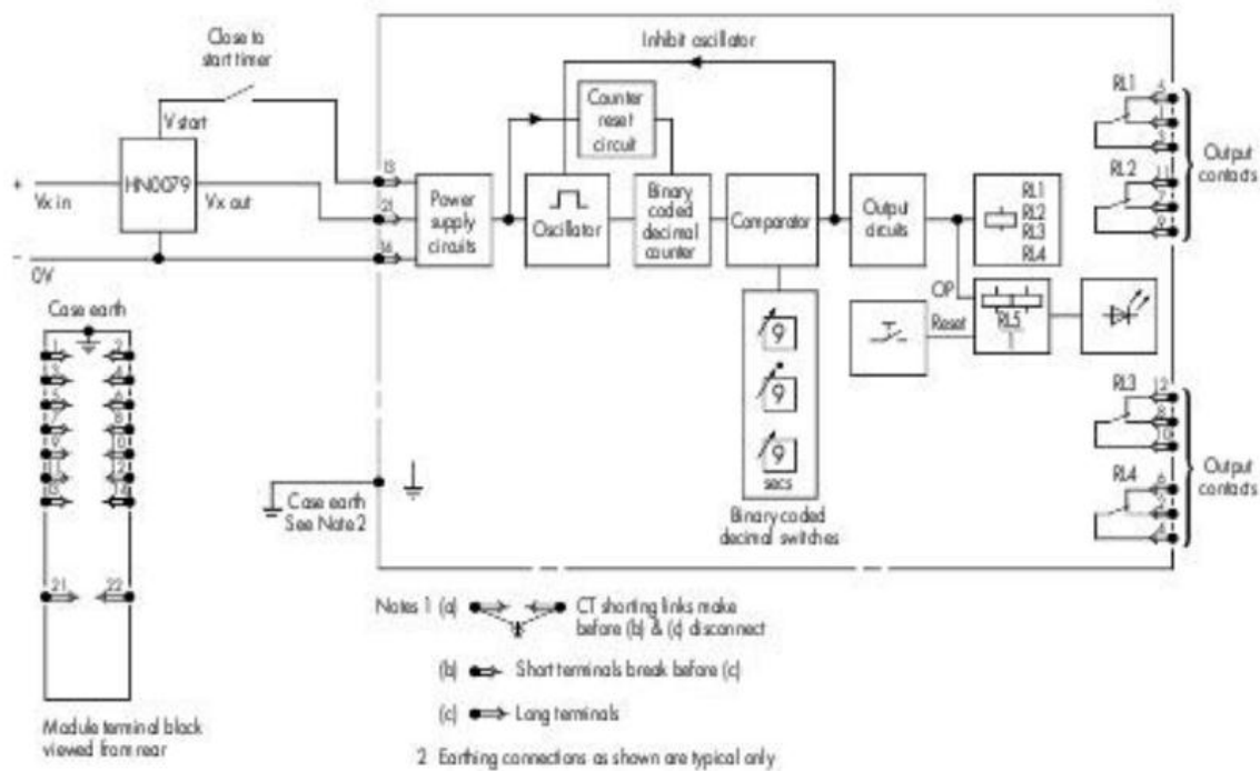
Figure 4 Application diagram: digital time delay relay type MVTT 14 220V (dc version)
