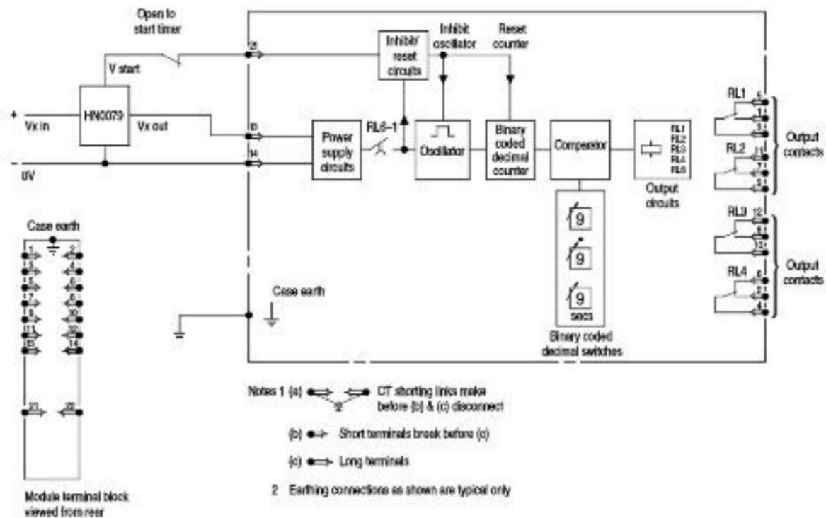
Figure 5 Application diagram: digital time delay relay, type MVTT 15 220V (dc version)
