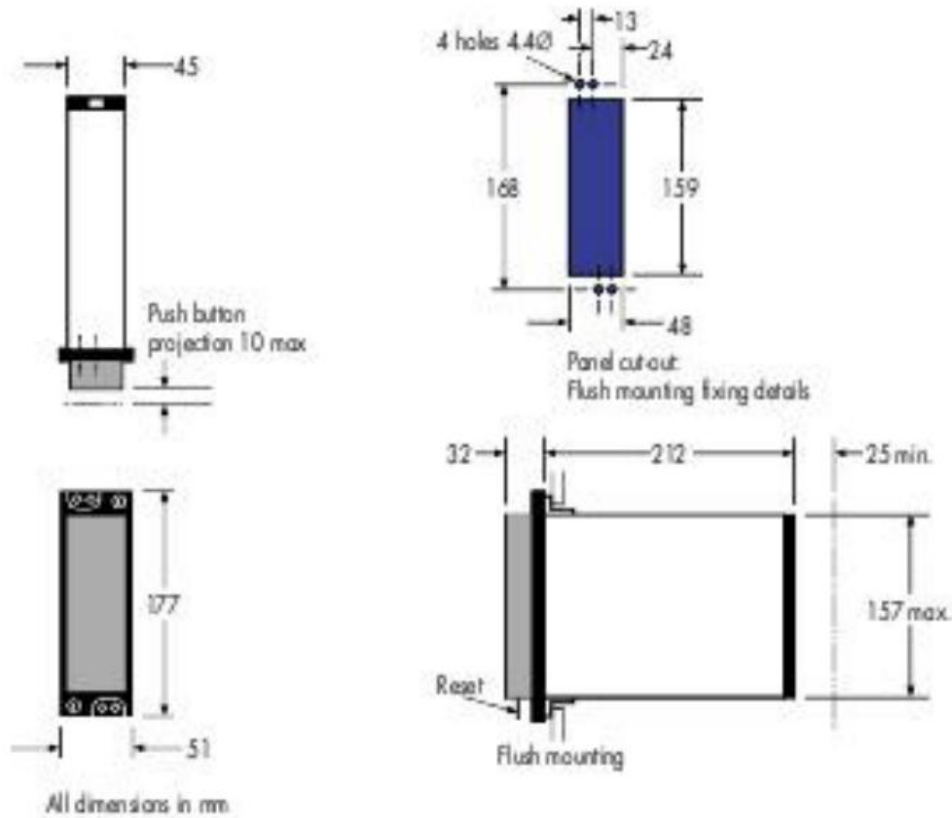
Figure 6 Case outline size 2
