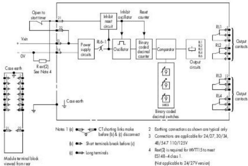
Figure 3 Application diagram: digital time delay relay type MVTT 15 (dc version)
